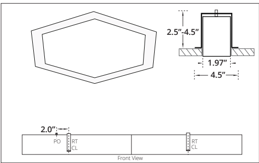
RECESSED TRIMLESS RT - Recessed Trimless Bracket PO - Power Opening CL - Center of Arm length *Cutout Dimensions = Total Length x Width of Extrusion.
