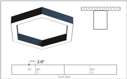
SURFACE MOUNT MH - Mounting Hole PO - Power Opening CL - Center of Arm length
