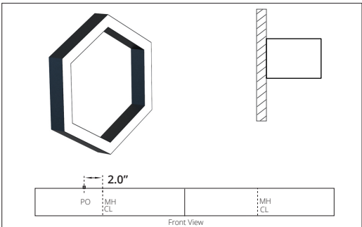
WALL FLUSH MH - Mounting Hole PO - Power Opening
