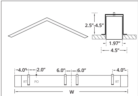
RECESSED TRIMLESS PO - Power Opening RT - Recessed Trimless Bracket 1. Cutout Dimensions = Arm Lengths x Width of Extrusion.
