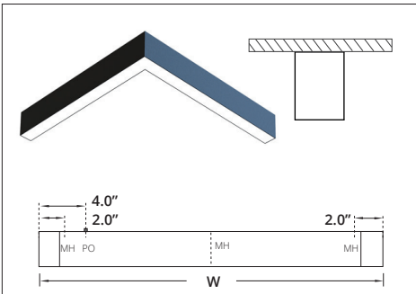
SURFACE MOUNT PO - Power Opening MH - Mounting Hole
